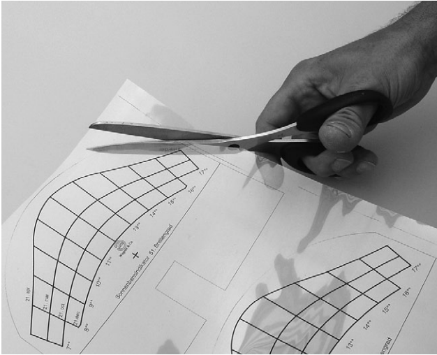
Figure 2: Select the correct sun path foil (e.g. 51° lat. = D, NL, B, Southern UK; 48° lat. = AU, CH etc., 53° lat. = IE, Northern UK), cut out the correct foil for your region along the thin markings and insert it into the stainless steel holder.
